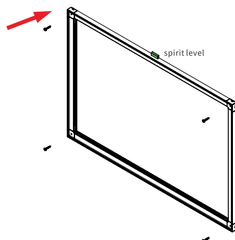
4. Secure frame to the wall using spirit level and screws (included).
